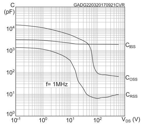
Figure 9: Capacitance variations
